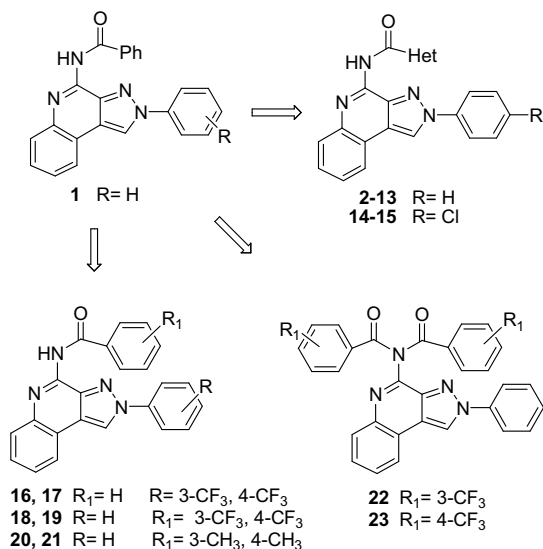
Chart 1. Previously and herein reported 2-arylpyrazolo[3,4-c]quinolin-4-amido derivatives.
