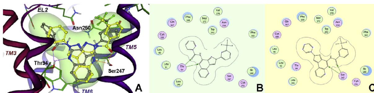
Figure 4. (A) Superimposition of 'A' docking conformation of compound 16 ( hA_3 K_i = 52 \pm 5 nM) and 'B' docking conformation of compound 18 ( hA_3 K_i = 60 \pm 8 nM); 18 is colored in yellow; H-bond interactions of 16 with hA_3 (Thr94 residue) are in lilac dash lines, while H-bond interactions of 18 with hA_3 (Ser247 residue) are in orange dash lines. (B) Schematic view of 16 'A' docking conformation within hA_3 binding site; H-bond interactions with Thr94 residue are indicated. (C) Schematic view of 18 'Bss' docking conformation within hA_3 binding site; H-bond interactions with Ser247 residue are indicated.
