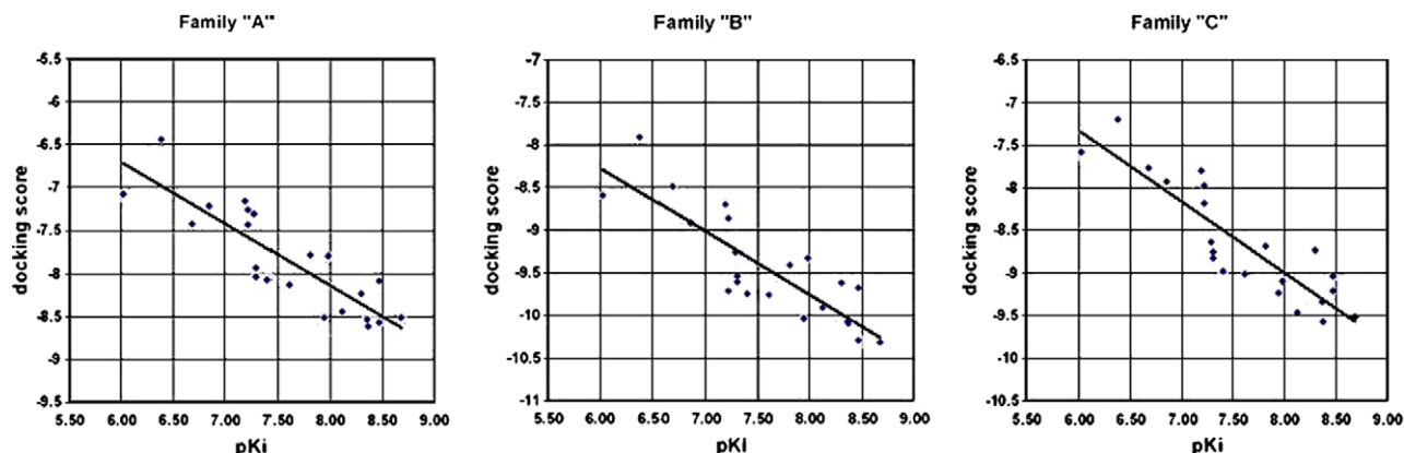
Figure 2. Left to right, experimental pK_i -docking score plots for the three conformation families. Docking scores in plots were calculated with MOE Affinity dG scoring function for minimized docking conformations (see Section 6 for details). Family A: average docking score = -7.85 ; correlation R^2 = 0.7412 . Family B: average docking score = -9.45 ; correlation R^2 = 0.7187 . Family C: average docking score = -8.66 ; correlation R^2 = 0.7568 .
