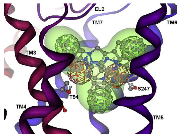
Figure 3. Superimposition of the three docking conformations of compound 1 (one conf. per family) and depiction of 3D pharmacophore. Three hydrophobic/aromatic features (green color) are located at peripheral points of Y-shaped binding site, while two H-bond acceptor features represent the two possible locations of the acceptors couple (the 4-arylamido carbonyl group substituent and the N5 atom) in proximity of Thr94 or Ser247 residues.
