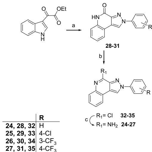
Scheme 1. Reagents and conditions: (a) arylhydrazine hydrochloride, absolute EtOH, AcOH, microwave irradiation; (b) PCl 5 /POCl 3 ; (c) NH 3 (g), absolute EtOH.
