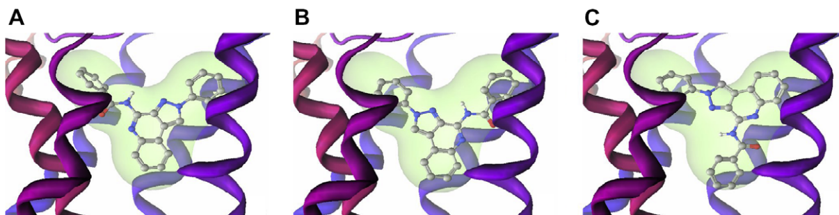
Figure 1. Left to right, in order A, B and C docking conformation families; the three docking conformations for compound 1 are shown.
